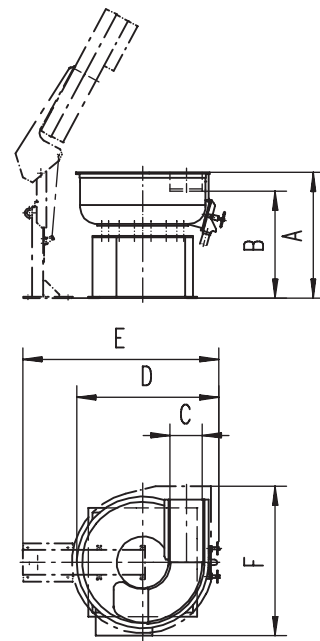
CD Circular vibrator with acoustic lid
